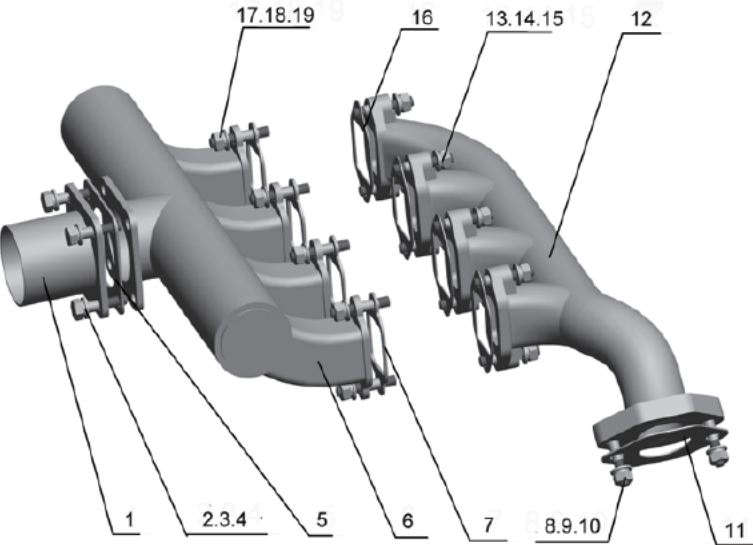
ENGINE- INTAKE AND EXHAUST MANIFOLD ASSY HY480-I
